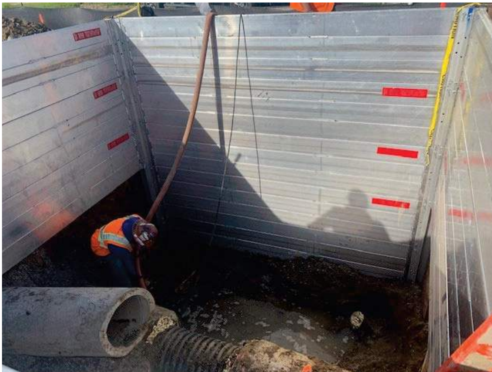
Figure 5 – Drainage System 2 – Shoring and Pumping Groundwater
