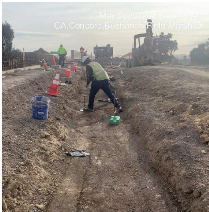
Figure 4 – Compaction Testing Drainage System 1
