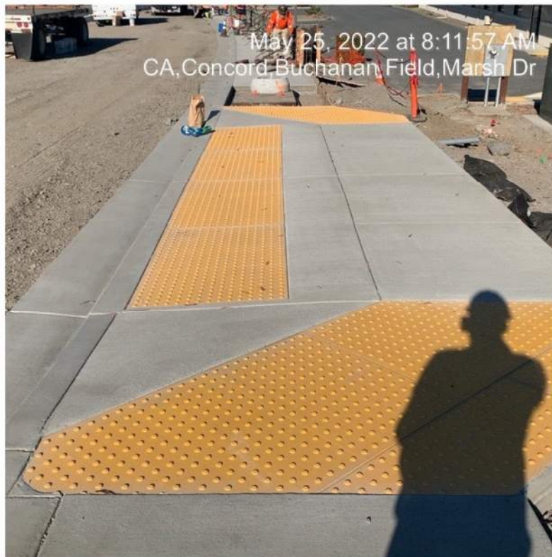
Figure 2 – Curb/ Gutter & Sidewalk at Access Road 2
