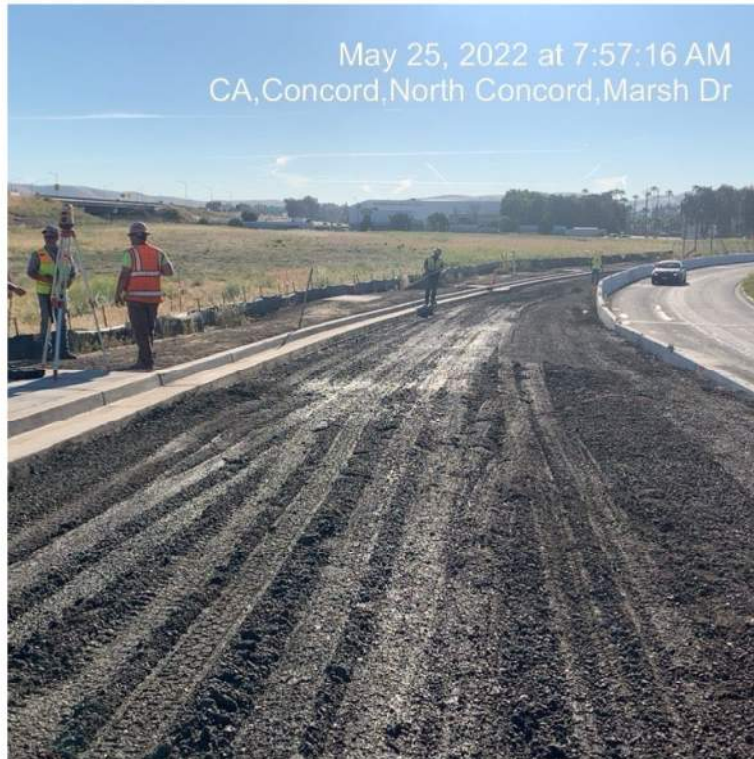
Figure 5 – Fine Grading Class 2 AB (East End of Bridge)
