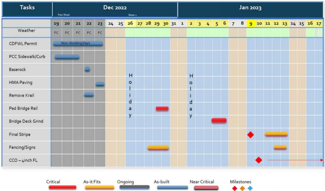
Figure 1 – Weekly Look-ahead Schedule
