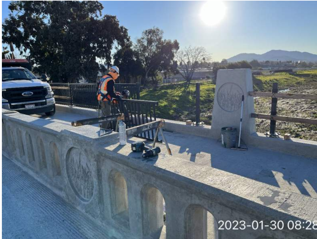
Figure 3 – Crew Installing Ped Rail at Pilasters
