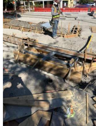
Fig. 2. - Installation of Drain Inlets/Formwork
