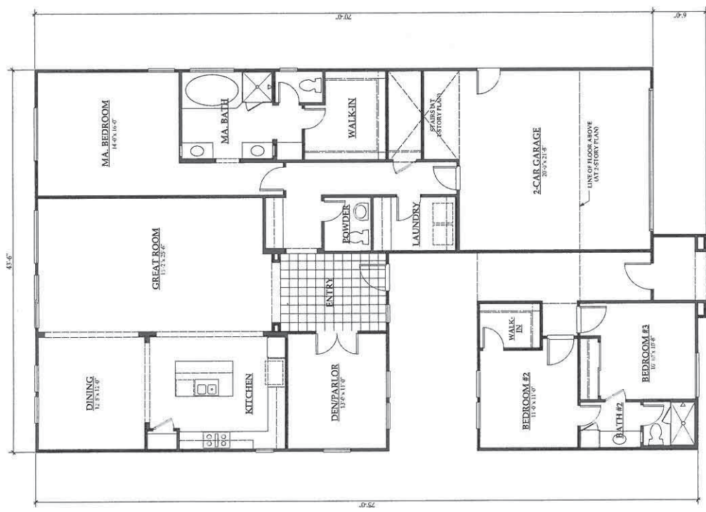
FLOOR PLAN (2276 S.F.)
